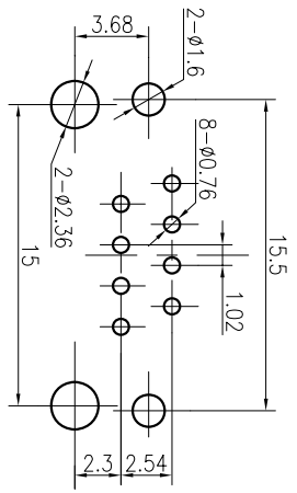
PC Board Layout
